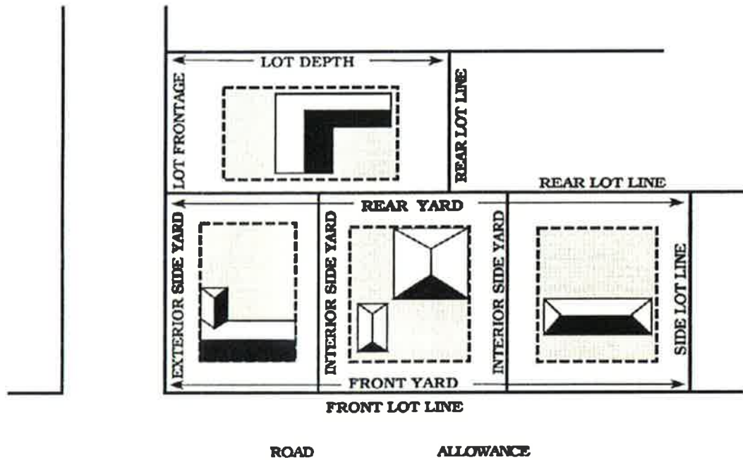
Figure 3.15: Yard Definitions
