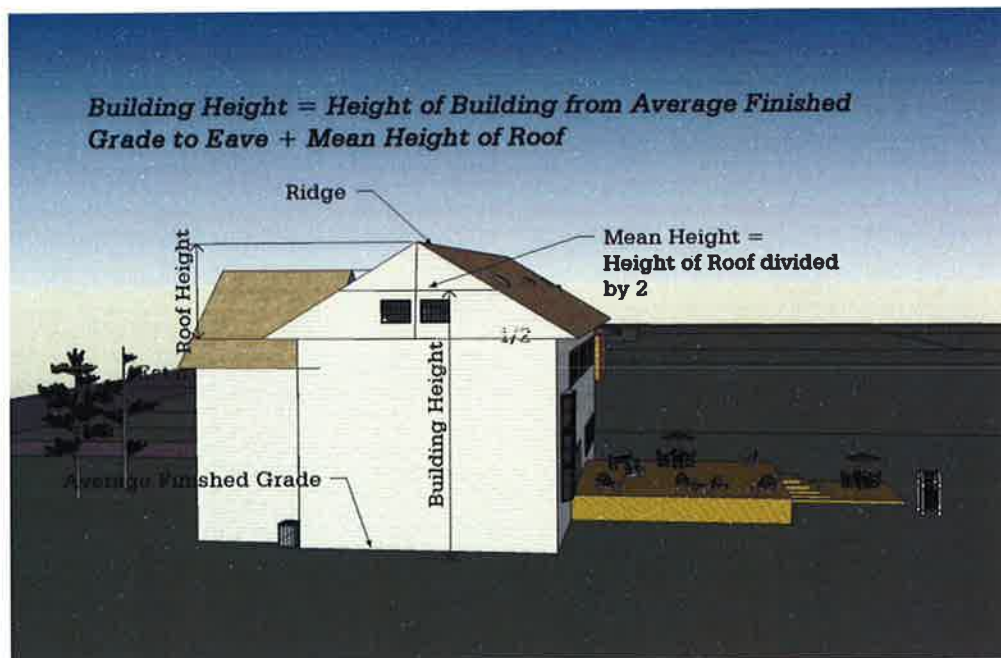
Figure 3.9: Building Height – All Other Roofs
